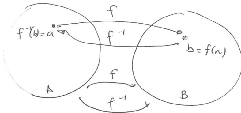
Figure 6: Inverse Functions
